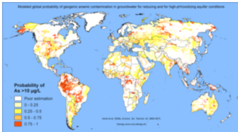
Modeled global probability of geogenic arsenic contamination in groundwater for reducing and for high-pH/oxidizing aquifer conditions.
