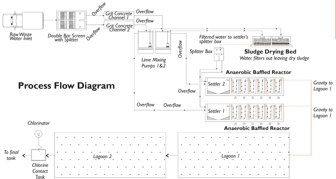
Figure 5. Typical layout of a permanent lime stabilization system.
