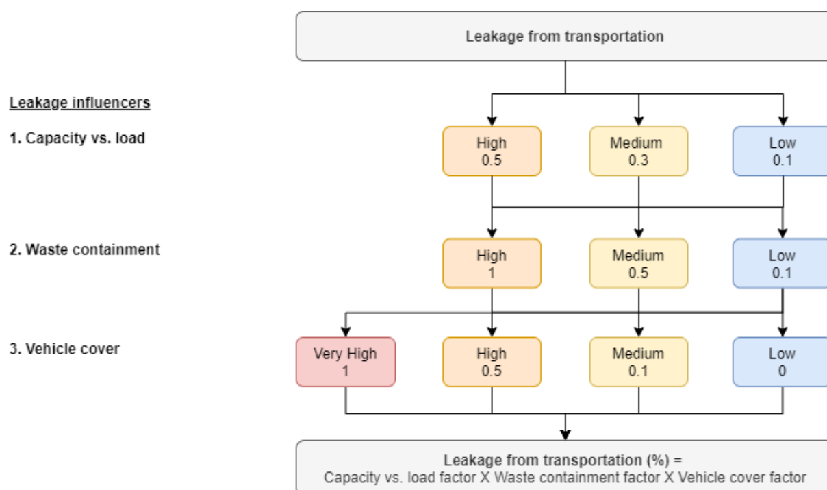
Figure 13: Decision tree and calculation of leakages from Transportation
